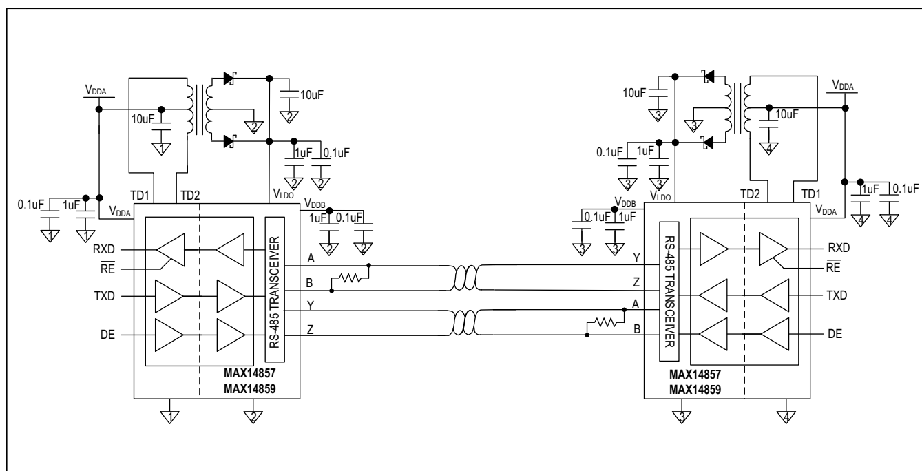
Figure 10. Typical Isolated RS-485/RS-422 Application with Integrated Transformer Driver
