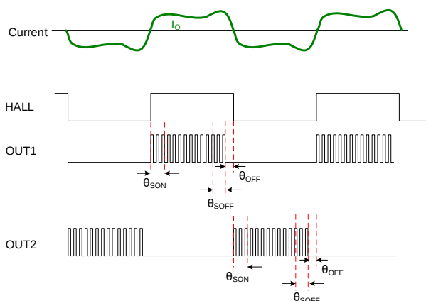
Figure 2: Timing Diagram
