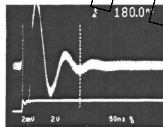
FIGURE 12: OP-61's Extremely Fast Recovery Time from a 1mA Load Transient to 0.01%
