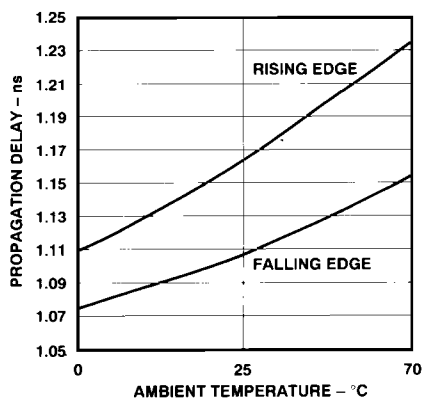
Figure 4. Driver Propagation Delay vs. Temperature
