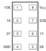
X2-DFN1210-8
