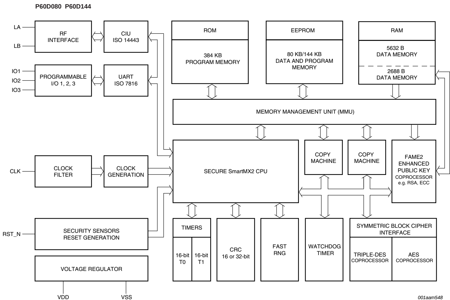
Fig 1. Functional diagram P60D080/P60D144
