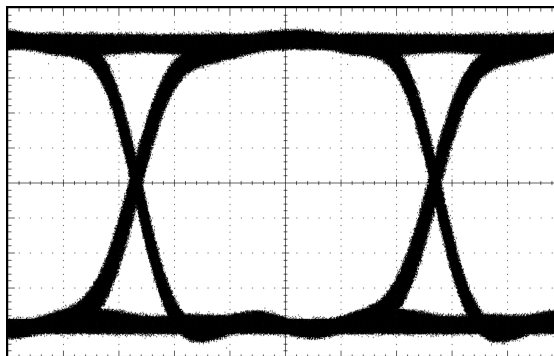
Cable Driver Output at 2.97 Gbps
