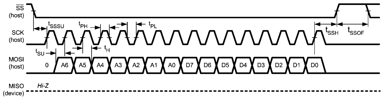
FIGURE 2. SPI Write
