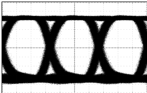
Equalizer Output at 2.97 Gbps with 120m Belden 1694A
