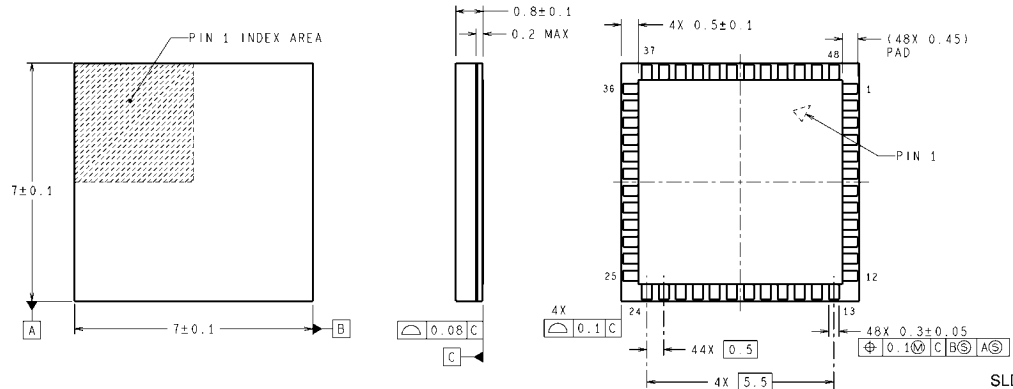
48-Pin Laminate TCSP Order Number LMH0387SL NS Package Number SLD48A
