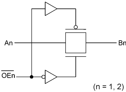
TC7WBL3306CFK
