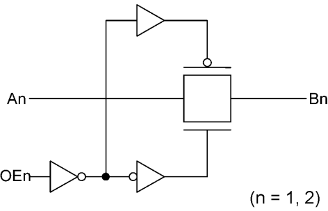
TC7WBL3305CFK
