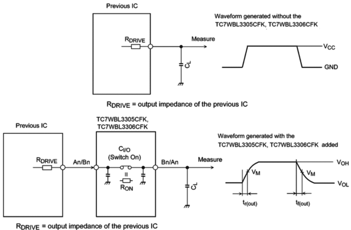
Fig. 12.1 Calculation Circuit
