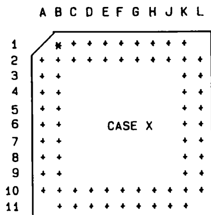
PIN SIDE VIEW *PIN 1
