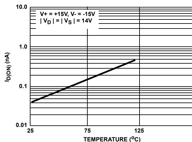
FIGURE 7. I_{D(ON)} vs TEMPERATURE (NOTE 11)
