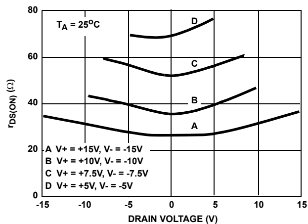
FIGURE 3. r_{DS(ON)} vs V_D
