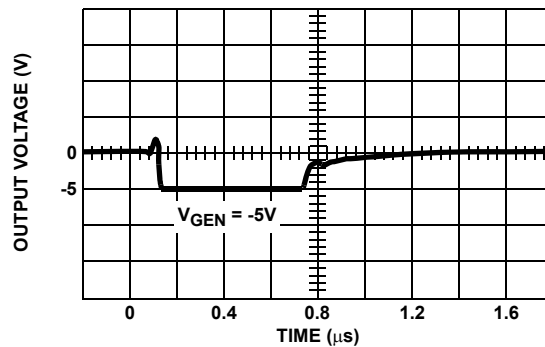
FIGURE 1F. V_{ANALOG} = -5V
