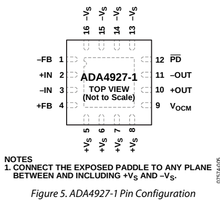
Figure 5. ADA4927-1 Pin Configuration
