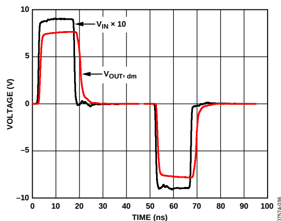
Figure 36. Overdrive Recovery, G = 10
