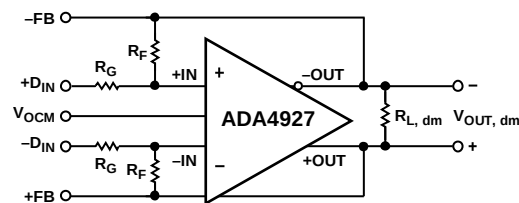
Figure 46. Circuit Definitions
