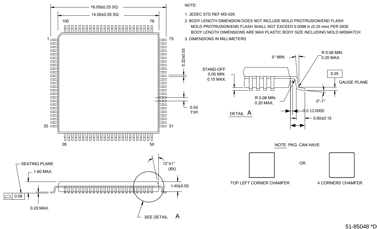
Figure 27. 100-Pin TQFP
