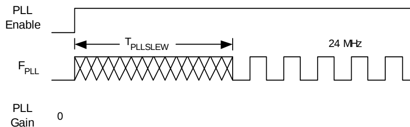
Figure 13. PLL Lock Timing Diagram
