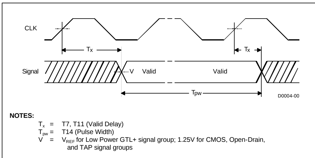
Figure 3.4 Valid Delay Timings
