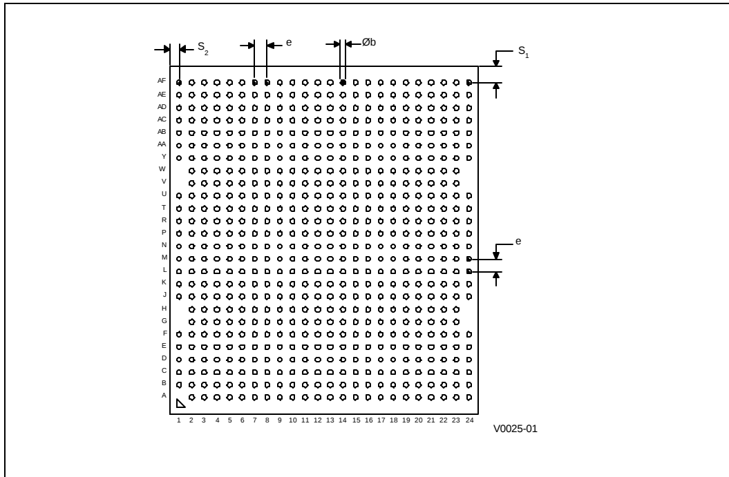
Figure 5.4 Surface-mount BGA Package - Bottom View
