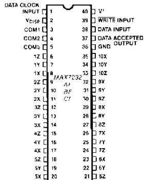
40 Lead DIP
