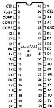
40 Lead DIP
