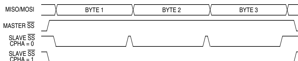
Figure 16-6. CPHA/SS Timing
