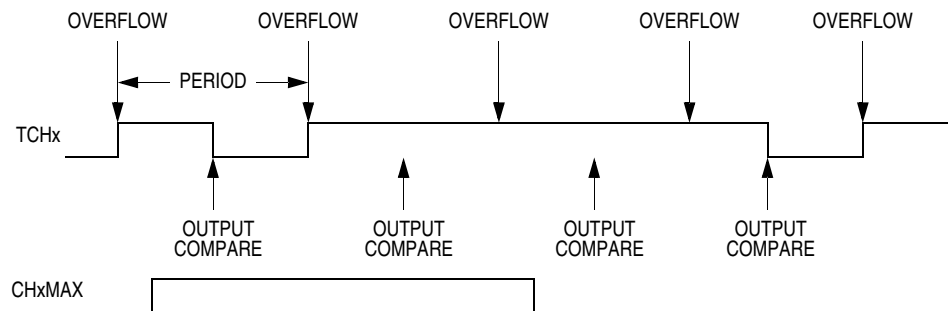
Figure 18-12. CHxMAX Latency
