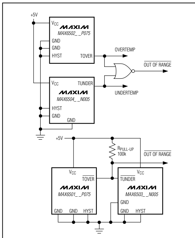
Figure 4. Temperature-Window Alarms
