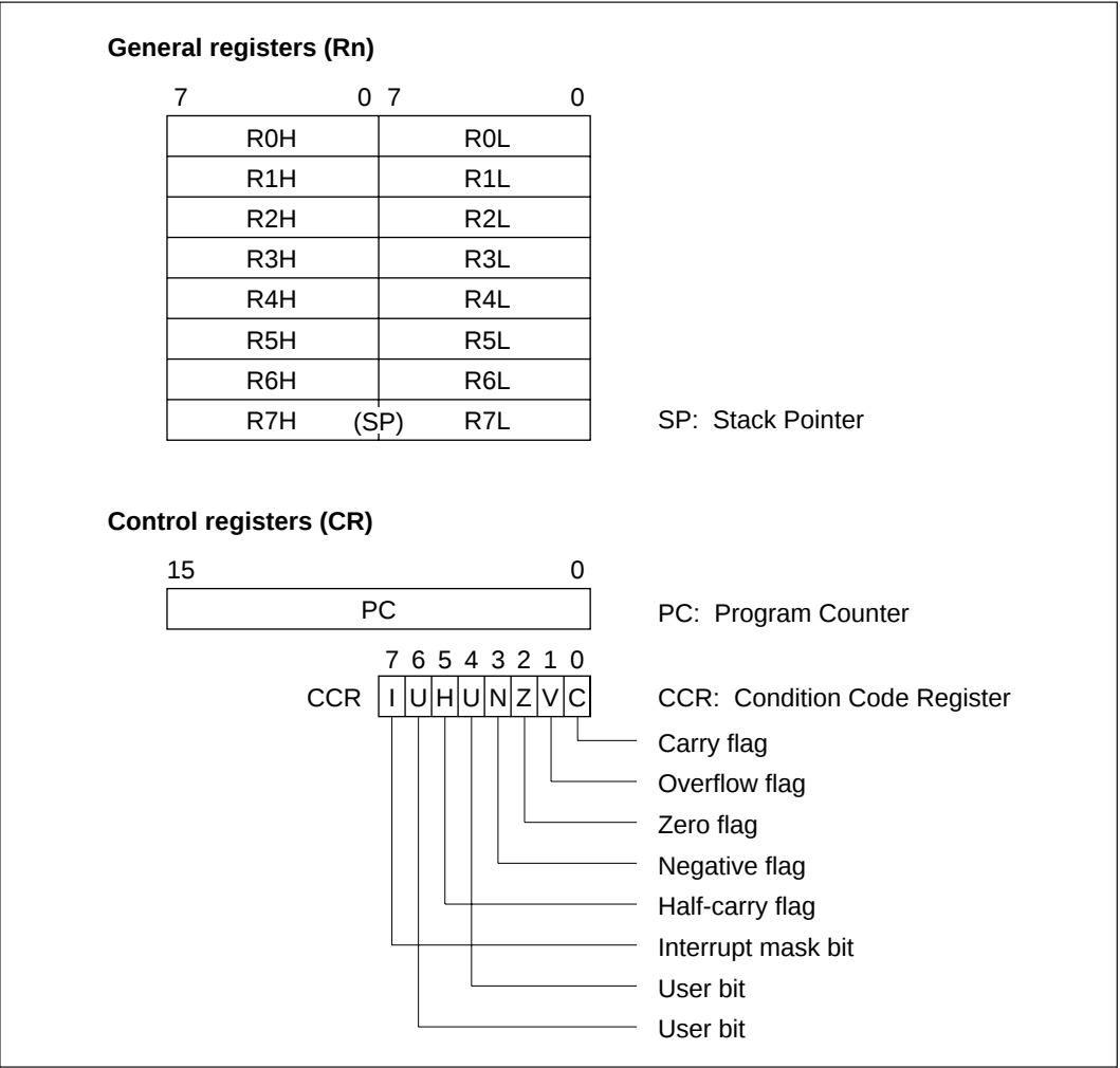
Figure 2-1 CPU Registers
