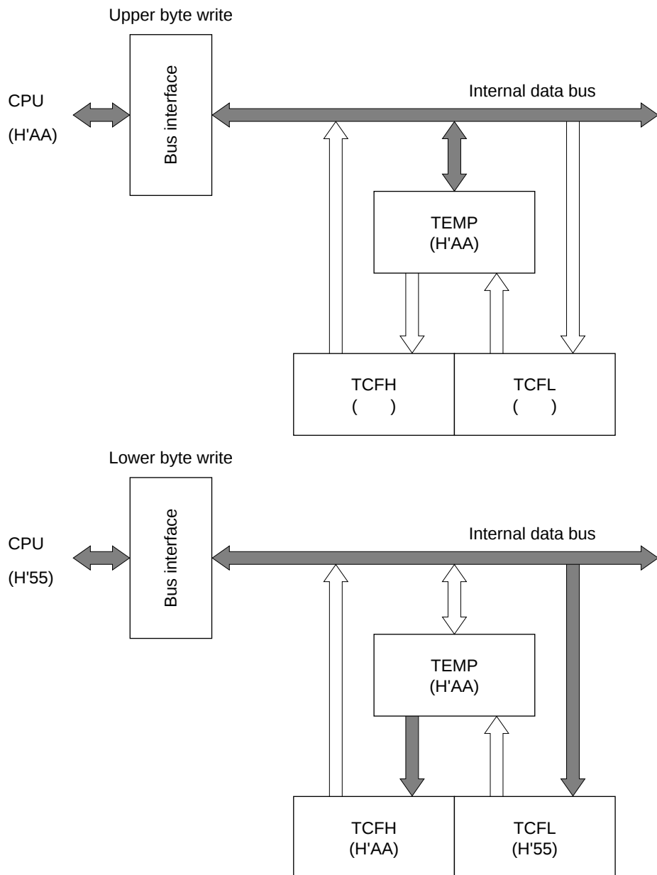
Figure 9-5-2 TCF Write Operation (CPU → TCF)
