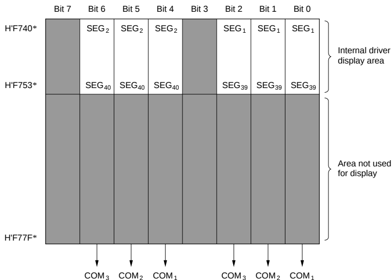
Figure 13-4 LCD RAM Map 2: No External Segment Expansion (1/3 Duty)
