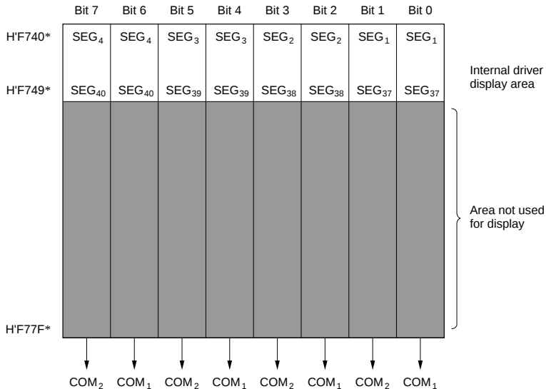
Figure 13-5 LCD RAM Map 3: No External Segment Expansion (1/2 Duty)
