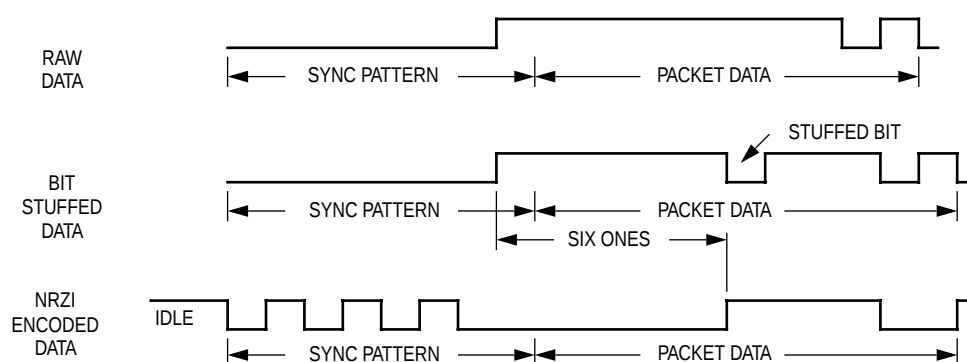
Figure 10-18. Bit Stuffing
