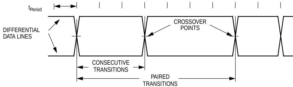
Figure 10-14. Data Jitter
