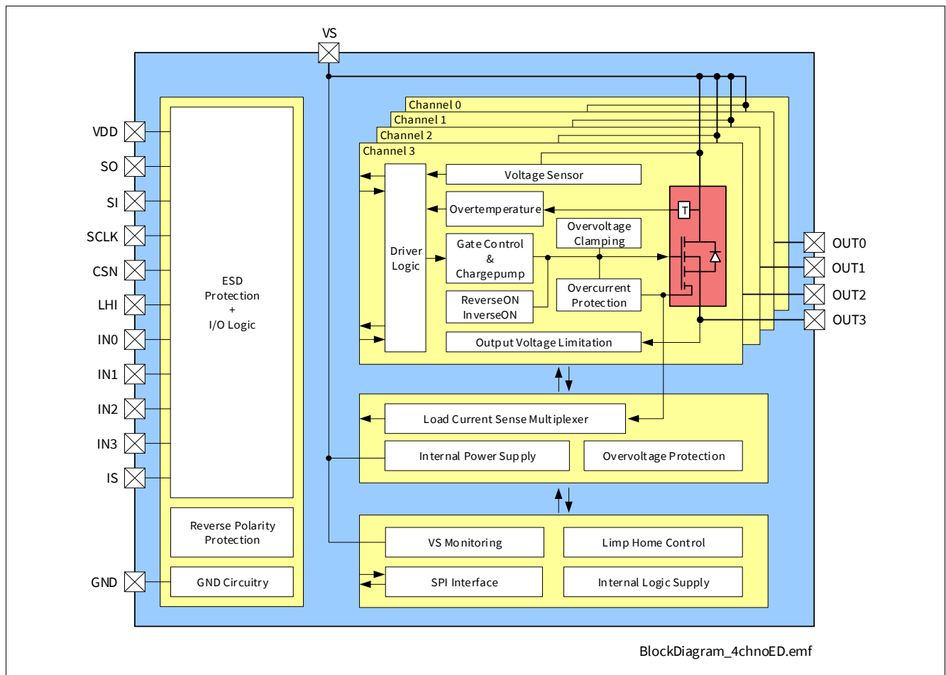
Figure 2 Block Diagram of BTS71040-4ESA
