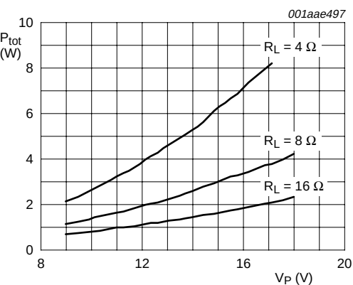
Fig 12. Total power dissipation (worst case, both channels driven) as a function of supply voltage
