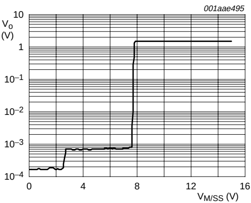
Fig 10. Output voltage as a function of voltage on pin M/SS
