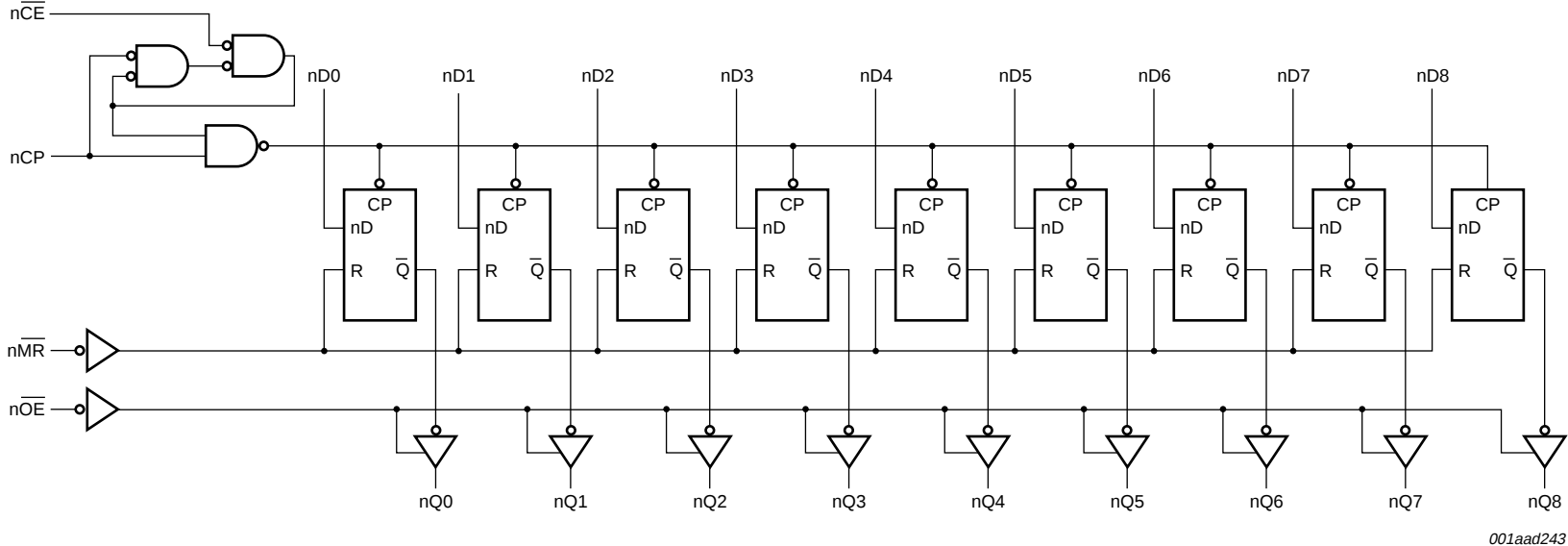
Fig 4. Logic diagram
