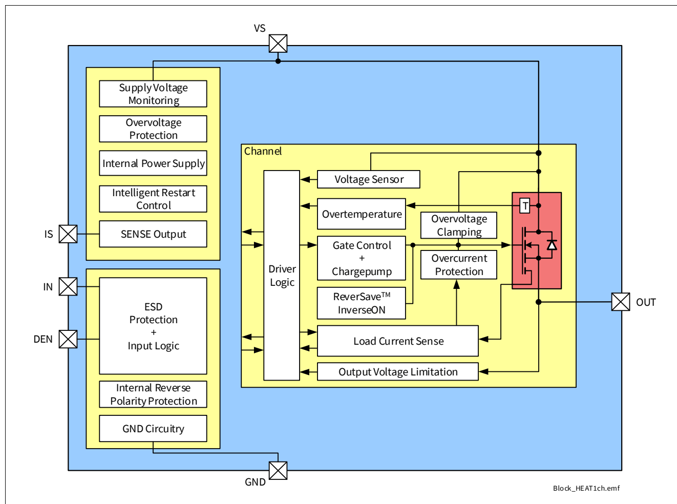
Figure 2 Block Diagram of BTS7008-1EPP
