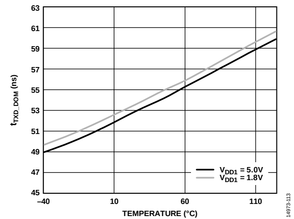
Figure 13. t_{TXD\_DOM} vs. Temperature ( R_{SLOPE} = 0 Ω)
