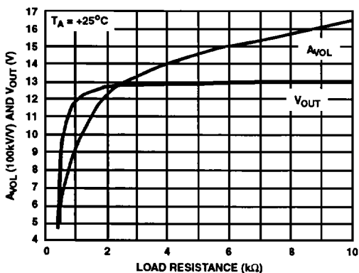
FIGURE 11. A_{VOL} AND V_{OUT} vs LOAD RESISTANCE
