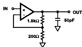
FIGURE 1. LARGE AND SMALL SIGNAL RESPONSE TEST CIRCUITS
