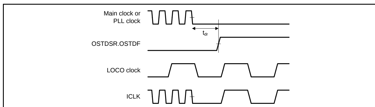
Figure 2.94 Oscillation Stop Detection Timing
