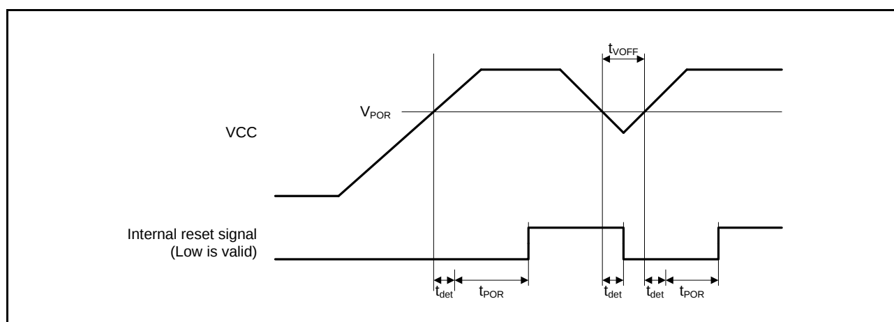
Figure 2.90 Power-on Reset Timing
