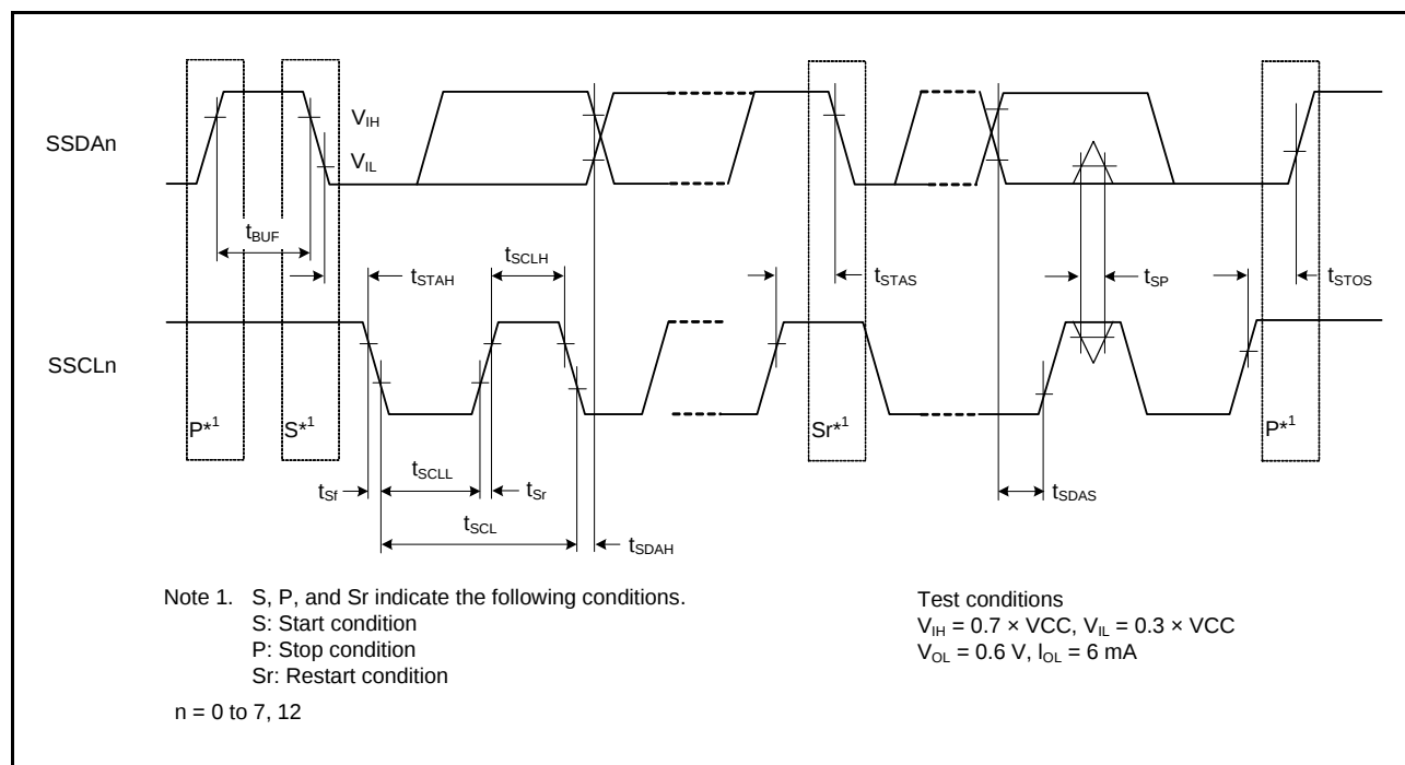
Figure 2.49 Simple IIC Bus Interface Input/Output Timing
