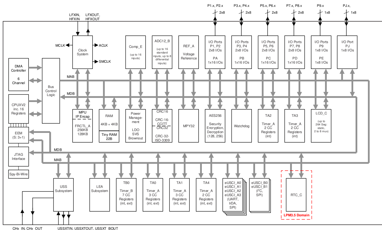
Figure 4-1. MSP430FR600x Functional Block Diagram
