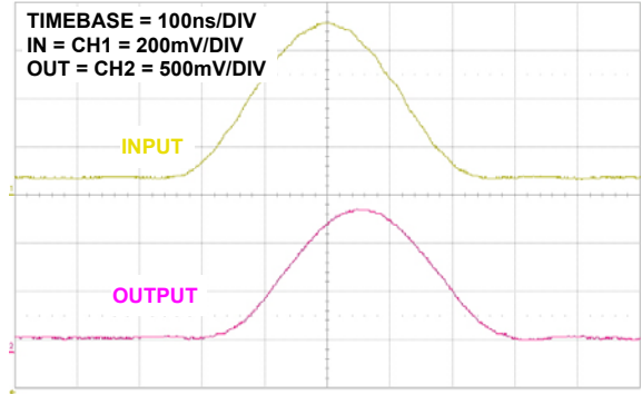
FIGURE 16. 2T RESPONSE
