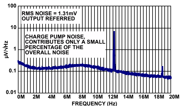
FIGURE 24. NOISE SPECTRUM
