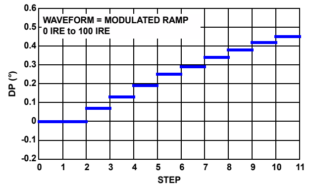
FIGURE 12. DIFFERENTIAL PHASE
