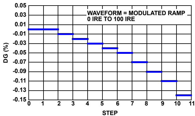
FIGURE 11. DIFFERENTIAL GAIN
