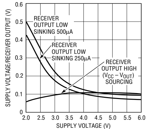
Receiver Output Voltage vs Supply Voltage
