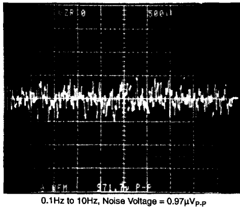
FIGURE 6. NOISE VOLTAGE ( A_v = 1000 )
