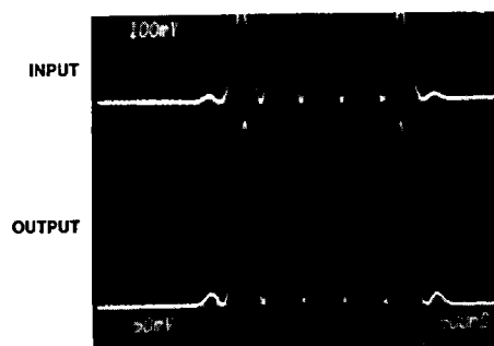
NTSC Method, R_L = 1k\Omega , C-L Delay < 7\text{ns} at T_A = +75^\circ\text{C} No Visual Difference at T_A = -55^\circ\text{C} or +125^\circ\text{C} Vertical Scale: Input = 100mV/Div., Output = 50mV/Div. Horizontal Scale: 500ns/Div.
