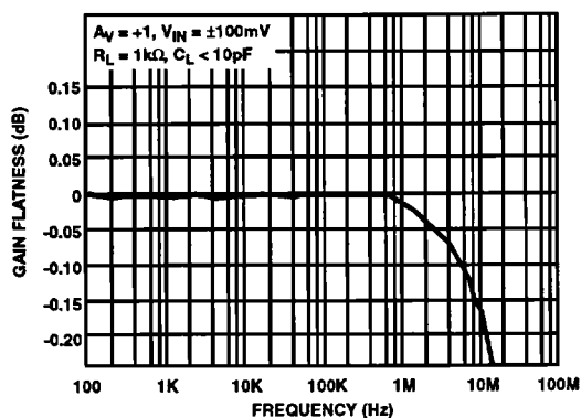
FIGURE 20. GAIN FLATNESS
