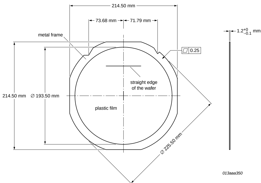
Fig 18. Film Frame Carrier (FFC) for 6 inch wafer (PCA2000U/10AC/1 and PCA2001U/10AC/1)
