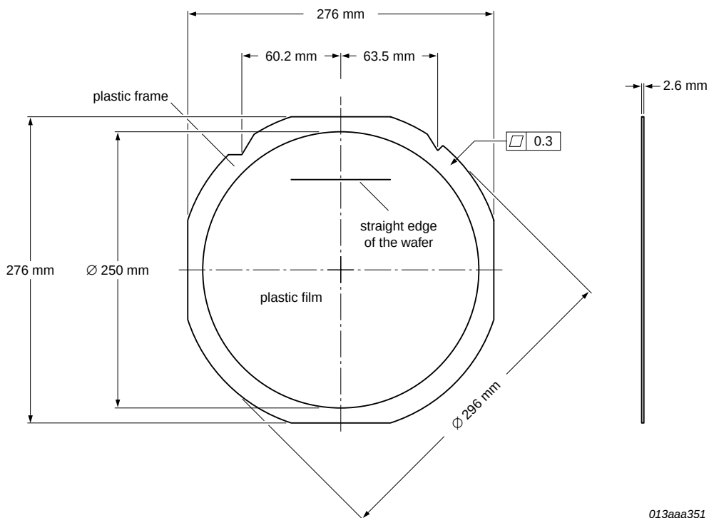
Fig 19. Film Frame Carrier (FFC) for 8 inch wafer (PCA2000CX8/12/1)
