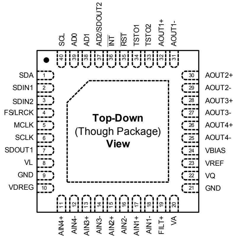
Figure 1. CS4244 Pinout
