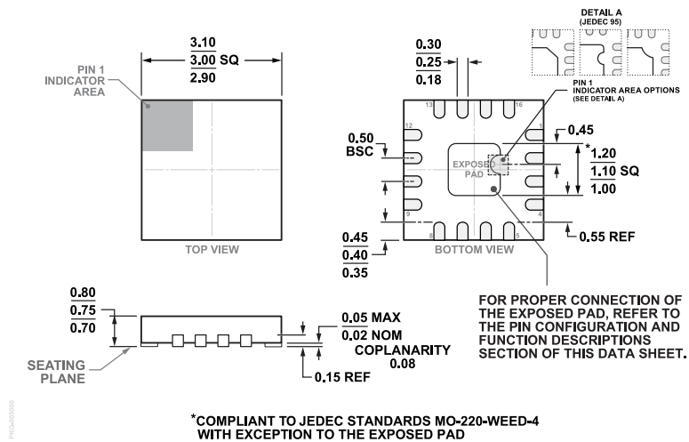
Figure 49. 16-Lead Lead Frame Chip Scale Package [LFCSP] 3 mm x 3 mm Body and 0.75 mm Package Height (CP-16-45) Dimensions shown in millimeters
