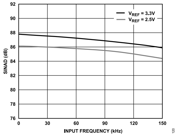
Figure 20. AD4685 SINAD vs. Input Frequency
