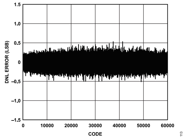
Figure 13. DNL Error
