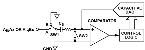
Figure 30. ADC Conversion Phase
