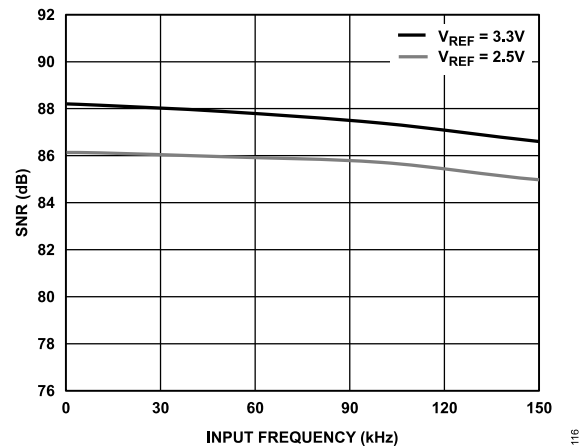
Figure 16. AD4685 SNR vs. Input Frequency
