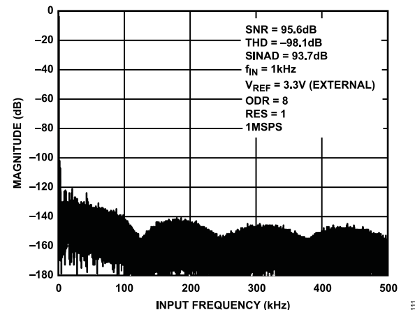
Figure 11. AD4684 FFT with Oversampling
