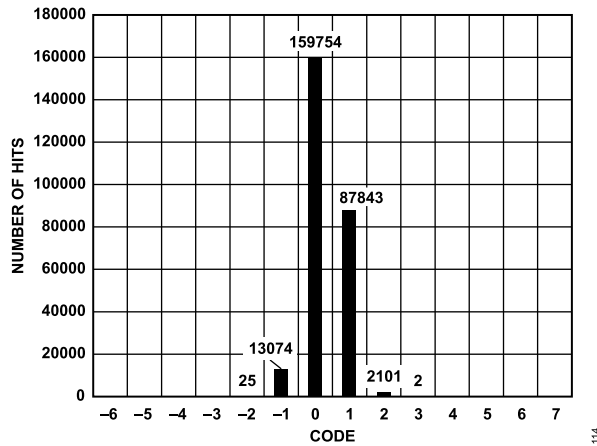
Figure 14. DC Histogram Codes at Code Center
