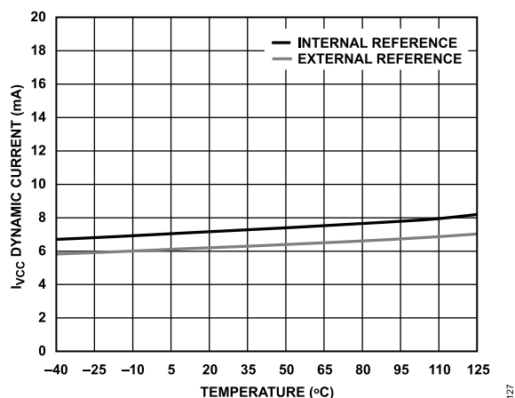
Figure 27. I_{VCC} Dynamic Current vs. Temperature
