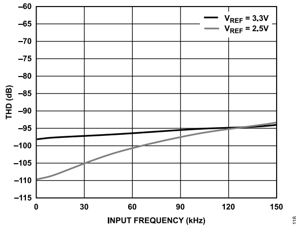
Figure 18. AD4685 THD vs. Input Frequency
