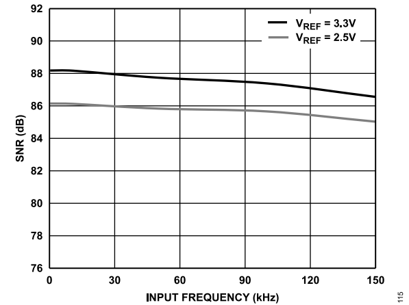
Figure 15. AD4684 SNR vs. Input Frequency
