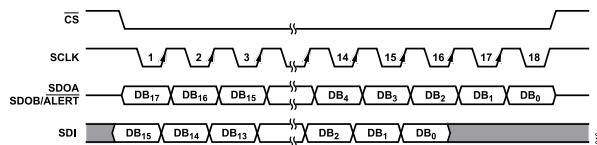
Figure 38. Resolution Boost
