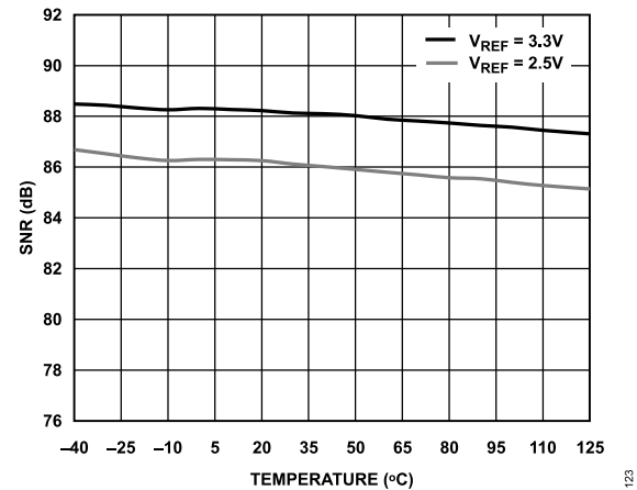
Figure 23. AD4685 SNR vs. Temperature
