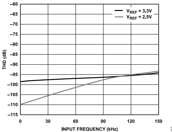
Figure 17. AD4684 THD vs. Input Frequency
