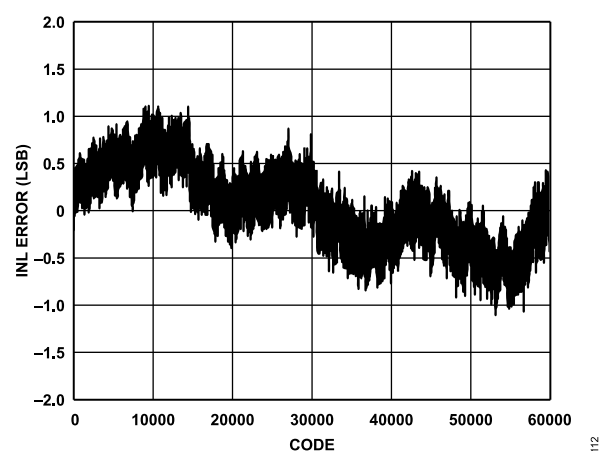
Figure 12. INL Error
