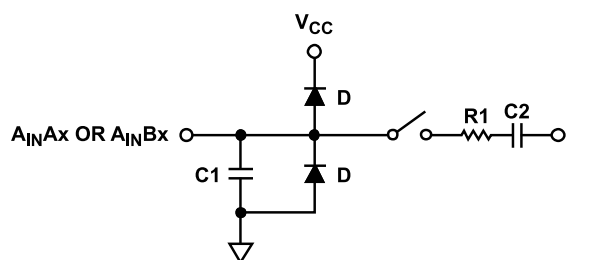
Figure 31. Equivalent Analog Input Circuit, Conversion Phase = Switch Open, Track Phase = Switch Closed
