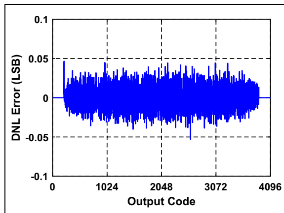
FIGURE 3-37: DNL Error vs. Output Code: f_S = 80 \text{ Msps} , f_{IN} = 4.3 \text{ MHz} , A_{IN} = -1 \text{ dBFS} .
