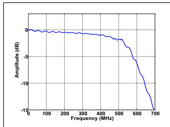
FIGURE 3-24: Input Bandwidth.
