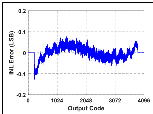
FIGURE 3-35: INL Error vs. Output Code: f_S = 80 \text{ Msps} , f_{IN} = 4.3 \text{ MHz} , A_{IN} = -1 \text{ dBFS} .
