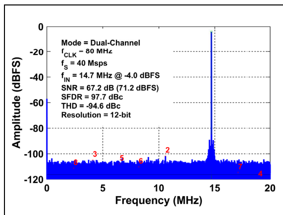
FIGURE 3-12: FFT for 14.7 MHz Input Signal: f_S = 40 Msps, Dual-Ch., A_{IN} = -4 dBFS.
