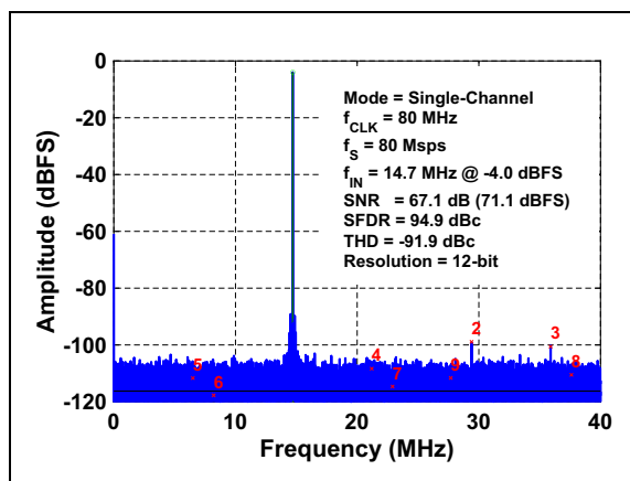
FIGURE 3-11: FFT for 14.7 MHz Input Signal: f_S = 80 Msps, Single-Ch., A_{IN} = -4 dBFS.
