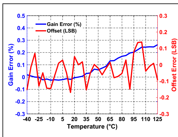
FIGURE 3-34: Gain and Offset Error Drifts vs. Temperature Using Internal Reference, with Respect to +25^{\circ}\text{C} : f_S = 80 Msp/s, A_{IN} = -1 dBFS.
