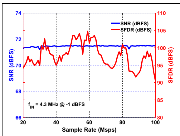
FIGURE 3-26: SNR/SFDR vs. Sample Rate (Mps): f_{IN} = 4.3 MHz, A_{IN} = -1 dBFS.
