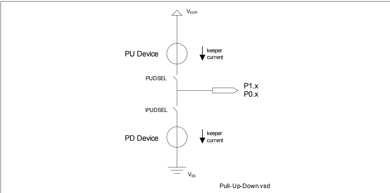
Figure 37 Pull-Up/Down Device
