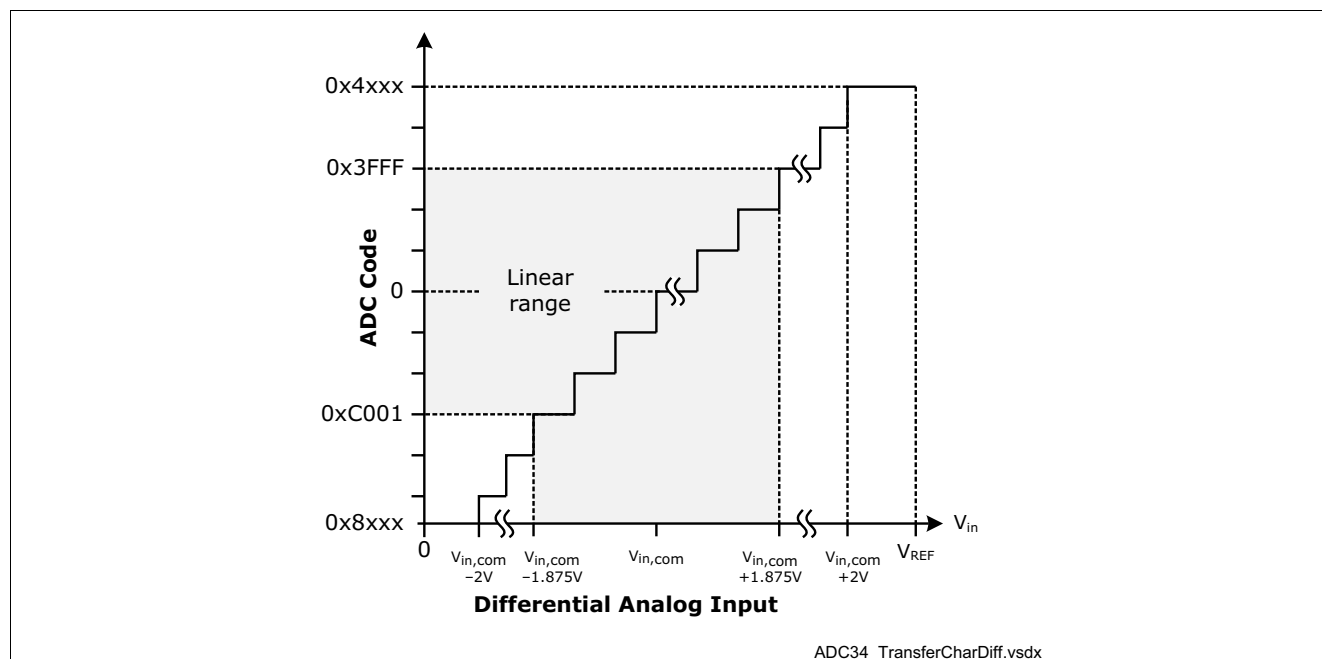
Figure 31 ADC output code over input voltage
