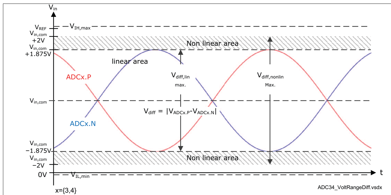
Figure 30 Input Voltage Range
