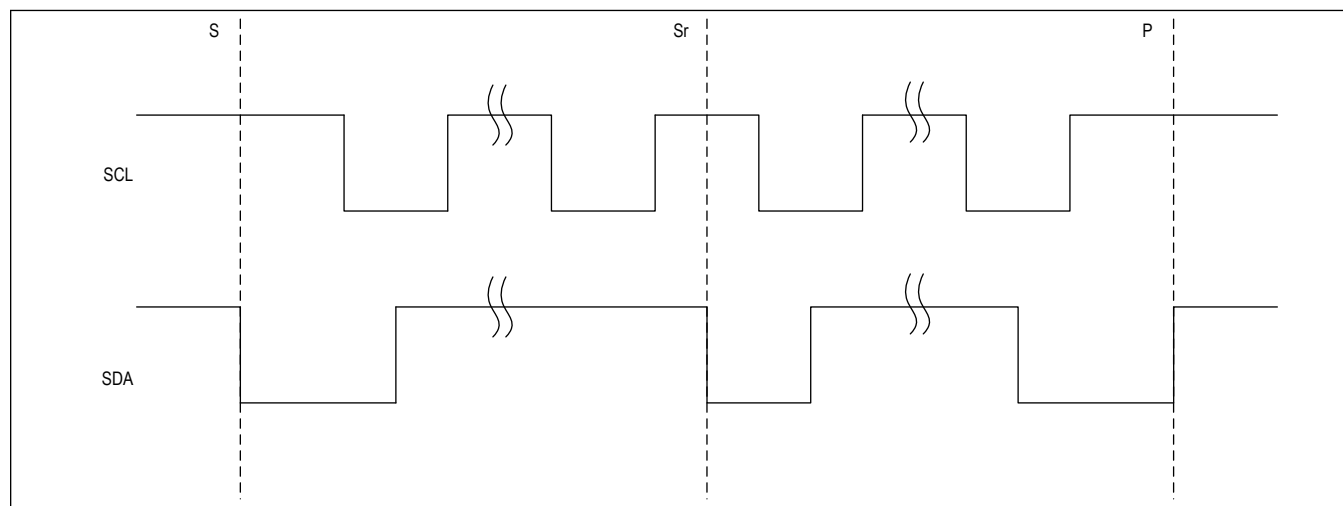
Figure 10. I^2C START, STOP, and REPEATED START Conditions
