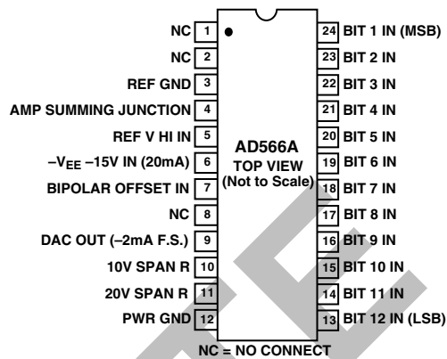
24-Lead DIP
