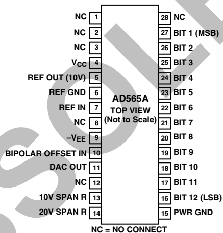
28-Lead SOIC
