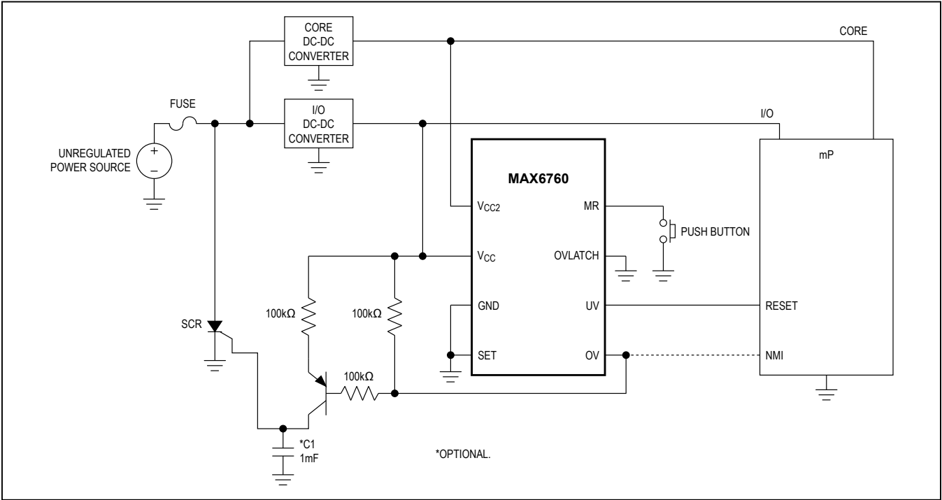
Figure 8. Microprocessor Monitoring
