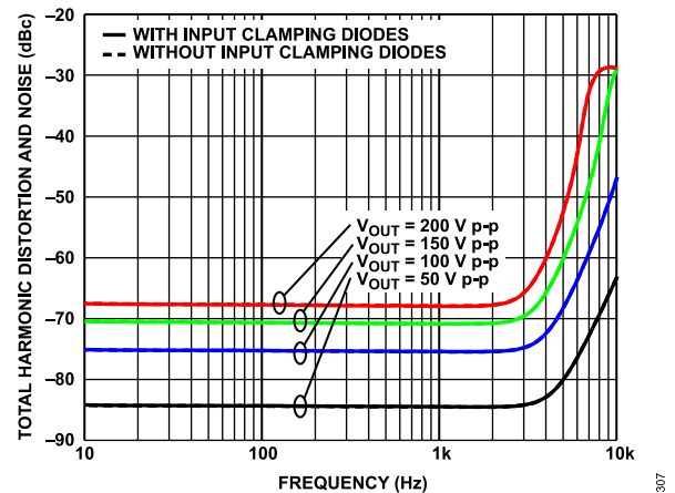
Figure 38. Total Harmonic Distortion and Noise vs. Frequency at Various Large Output Swings, T_A = 25^\circ\text{C} , A_V = 40 , V_S = \pm 110 V, R_F = 100 k \Omega , R_{LOAD} = 10 k \Omega , R_{ADJ} = 0 \Omega
