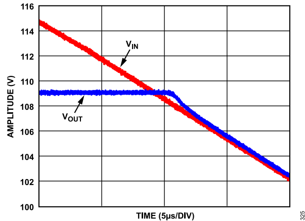
Figure 43. Output Overdrive Recovery, V_S = \pm 110 V, A_V = 40 , R_{LOAD} = 10 k \Omega , R_{ADJ} = 0 \Omega
