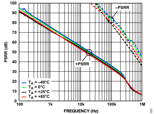
Figure 42. PSRR vs. Frequency at Various T_A , V_S = \pm 110 V, R_{LOAD} = 10 k \Omega , R_{ADJ} = 0 \Omega
