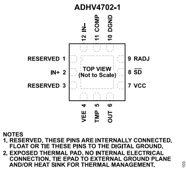
Figure 2. Pin Configuration
