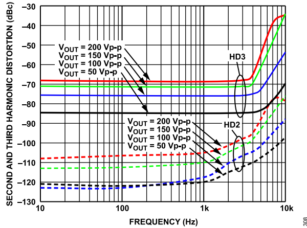
Figure 39. Second Harmonic Distortion (HD2) and Third Harmonic Distortion (HD3) vs. Frequency at Various Output Swings, T_A = 25^\circ\text{C} , A_V = 20 , V_S = \pm 110 V, R_F = 100 k \Omega , R_{LOAD} = 10 k \Omega , R_{ADJ} = 0 \Omega
