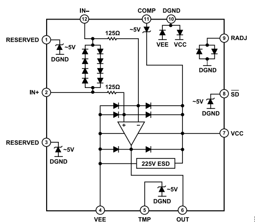
Figure 45. Simplified ESD Configuration
