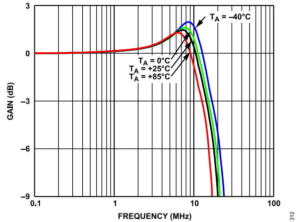
Figure 24. Small Signal Frequency Response at Various T_A , A_V = 1 , V_S = \pm 110\text{ V} , V_{OUT} = 100\text{ mV p-p} , R_L = 10\text{ k}\Omega , R_{ADJ} = 0\text{ }\Omega
