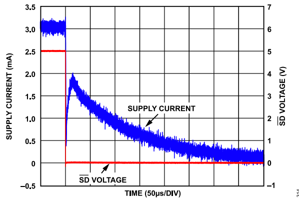
Figure 54. \overline{\text{SD}} Pin Response Time, Turning Off
