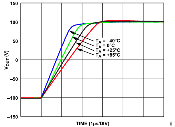
Figure 12. Large Signal Pulse Response at Various T_A , Rising Edge, A_V = 20 , V_S = \pm 110 V, V_{OUT} = 200 V p-p, R_F = 100 k \Omega , R_{LOAD} = 10 k \Omega , R_{ADJ} = 0 \Omega
