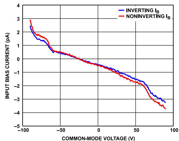
Figure 29. Input Bias Current vs. Common-Mode Voltage, T_A = 25^\circ\text{C} , V_S = \pm 110\text{ V} , R_{ADJ} = 0\ \Omega
