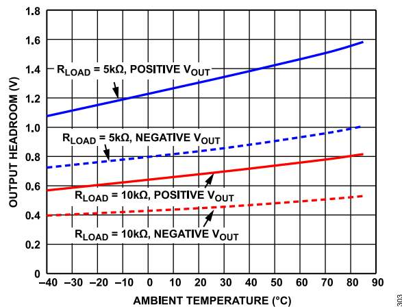
Figure 35. Output Headroom vs. Ambient Temperature at Various R_{LOAD} , V_S = \pm 110 V, R_{ADJ} = 0 \Omega
