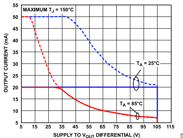
Figure 62. DC SOA at T_A = 25^\circ\text{C} and T_A = 85^\circ\text{C} , A_V = 20 , V_S = \pm 110\text{ V} , R_F = 100\text{ k}\Omega , R_{\text{ADJ}} = 0\text{ }\Omega
