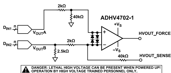
Figure 63. ADHV4702-1 Configured as a Voltage Subtractor Using DACs
