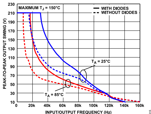
Figure 61. Dynamic SOA at T_A = 25^\circ\text{C} and T_A = 85^\circ\text{C} With and Without Input Clamping Diodes, A_V = 20 , V_S = \pm 110\text{ V} , R_F = 100\text{ k}\Omega , R_{\text{LOAD}} = 10\text{ k}\Omega , R_{\text{ADJ}} = 0\text{ }\Omega
