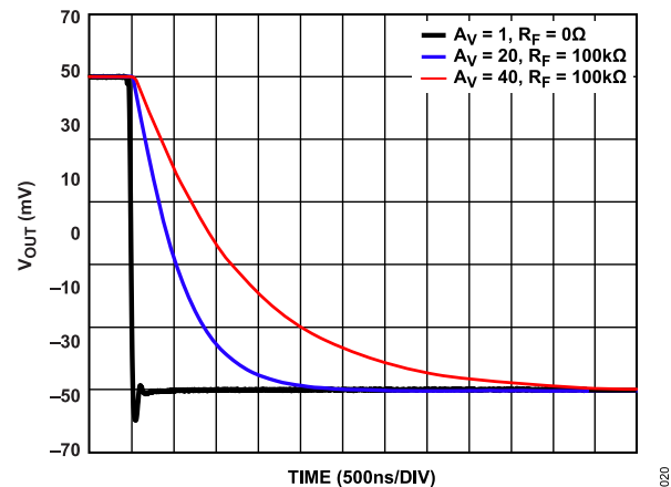
Figure 26. Small Signal Pulse Response at Various Gains, Falling Edge, T_A = 25^\circ\text{C} , V_S = \pm 110\text{ V} , V_{OUT} = 100\text{ mV p-p} , R_{LOAD} = 10\text{ k}\Omega , R_{ADJ} = 0\text{ }\Omega
