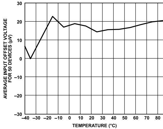
Figure 9. Average Input Offset Voltage for 50 Devices vs. Temperature, V_S = \pm 110 V
