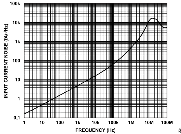
Figure 33. Input Current Noise vs. Frequency
