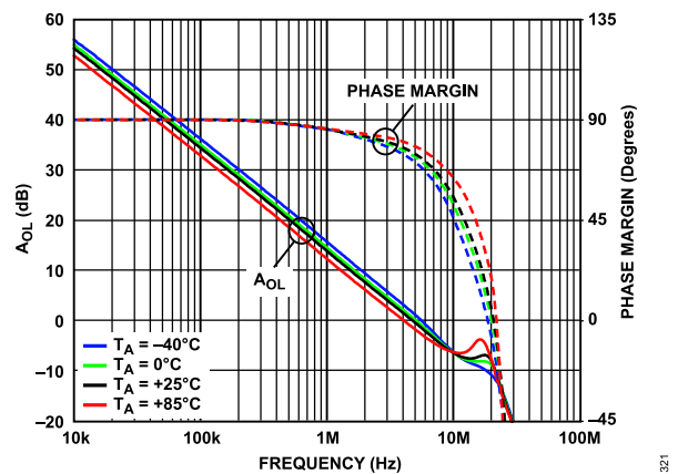
Figure 13. A_{OL} and Phase Margin vs. Frequency at Various T_A , V_S = \pm 110 V, R_{ADJ} = 0 \Omega
