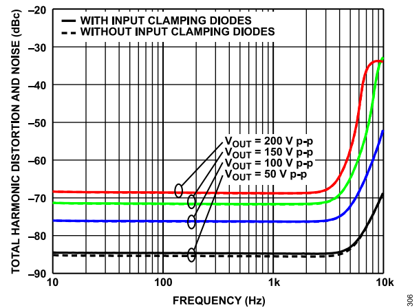
Figure 37. Total Harmonic Distortion and Noise vs. Frequency at Various Large Output Swings, T_A = 25^\circ\text{C} , A_V = 20 , V_S = \pm 110 V, R_F = 100 k \Omega , R_{LOAD} = 10 k \Omega , R_{ADJ} = 0 \Omega
