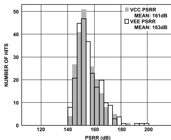
Figure 7. PSRR Distribution, T_A = 25^\circ\text{C} , V_S = \pm 110\text{ V} , R_{ADJ} = 0\ \Omega
