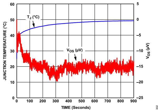
Figure 34. Offset Voltage Warmup Drift and T_J , V_S = \pm 110 , R_{ADJ} = 0 \Omega
