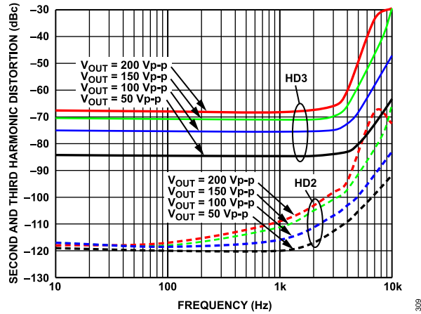
Figure 40. Second Harmonic Distortion (HD2) and Third Harmonic Distortion (HD3) vs. Frequency at Various Output Swings, T_A = 25^\circ\text{C} , A_V = 40 , V_S = \pm 110 V, R_F = 100 k \Omega , R_{LOAD} = 10 k \Omega , R_{ADJ} = 0 \Omega
