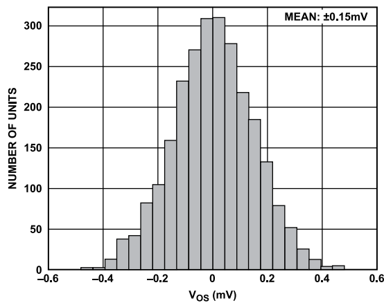
Figure 10. Input Offset Voltage Distribution, T_A = 25^\circ\text{C} , V_S = \pm 110 V, V_{CM} = 0 V, R_{ADJ} = 0 \Omega
