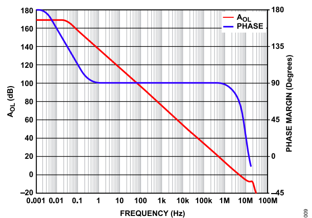
Figure 14. A_{OL} and Phase Margin vs. Frequency, T_A = 25^\circ\text{C} , V_S = \pm 110 V, R_{ADJ} = 0 \Omega
