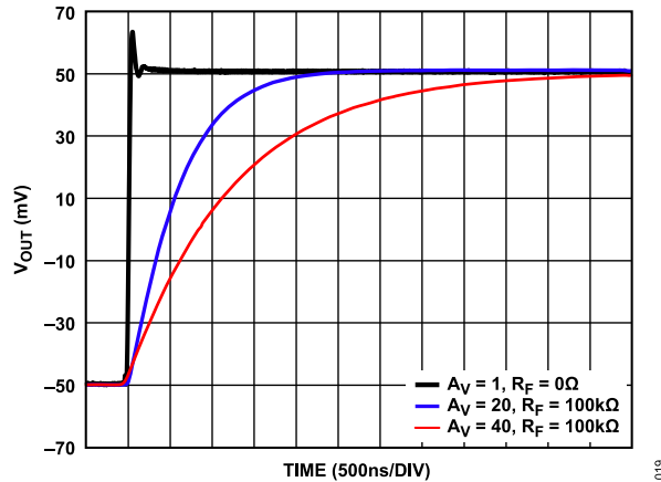
Figure 23. Small Signal Pulse Response at Various Gains, Rising Edge, T_A = 25^\circ\text{C} , V_S = \pm 110\text{ V} , V_{OUT} = 100\text{ mV p-p} , R_{LOAD} = 10\text{ k}\Omega , R_{ADJ} = 0\text{ }\Omega
