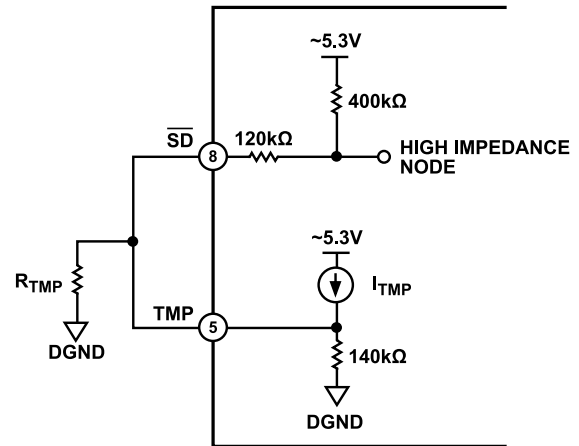
Figure 56. TMP and \overline{\text{SD}} Pin Configuration for Short-Circuit Protection and Thermal Shutdown
