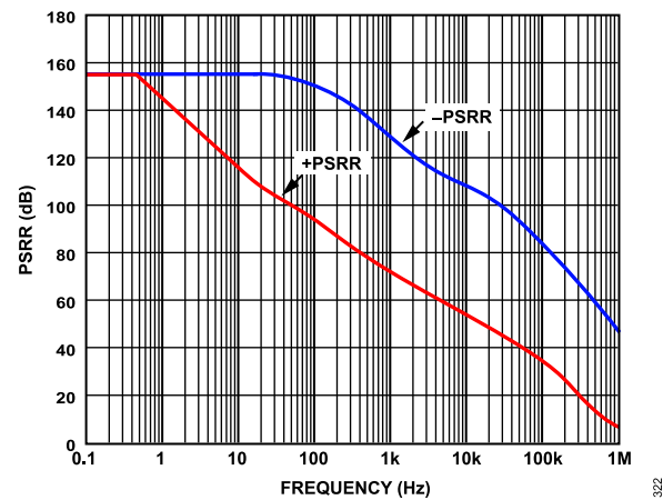
Figure 41. PSRR vs. Frequency, T_A = 25^\circ\text{C} , V_S = \pm 110 V, R_{LOAD} = 10 k \Omega , R_{ADJ} = 0 \Omega
