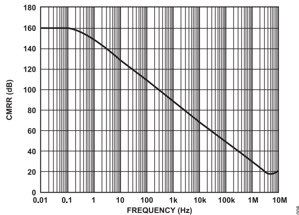
Figure 11. CMRR vs. Frequency, T_A = 25^\circ\text{C} , V_S = \pm 110 V, R_{LOAD} = 10 k \Omega , R_{ADJ} = 0 \Omega
