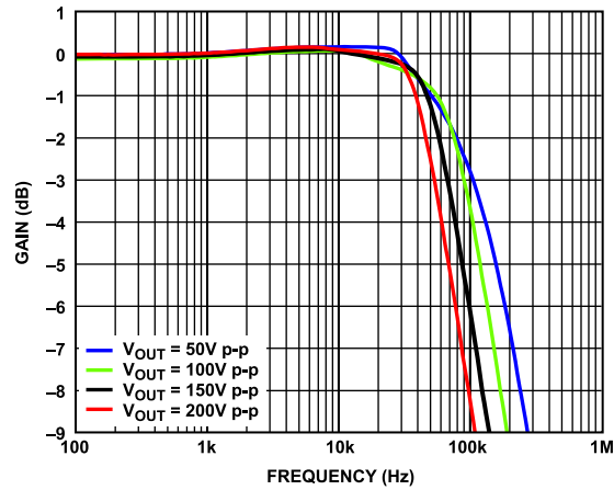
Figure 22. Large Signal Frequency Response at Various Output Swings with Input Clamping Diodes (See the Slew Boost Circuit and Protection Section ), T_A = 25^\circ\text{C} , A_V = 20 , V_S = \pm 110\text{ V} , R_F = 100\text{ k}\Omega , R_{LOAD} = 10\text{ k}\Omega , R_{ADJ} = 0\text{ }\Omega
