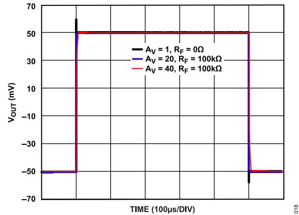
Figure 25. Small Signal Pulse Response at Various Gains, T_A = 25^\circ\text{C} , V_S = 110\text{ V} , V_{OUT} = 100\text{ mV p-p} , R_{LOAD} = 10\text{ k}\Omega , R_{ADJ} = 0\text{ }\Omega
