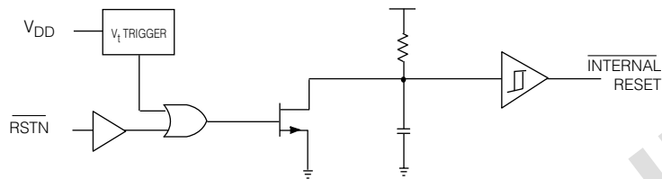
Fig. 2a GS9001 Internal Reset Circuit
