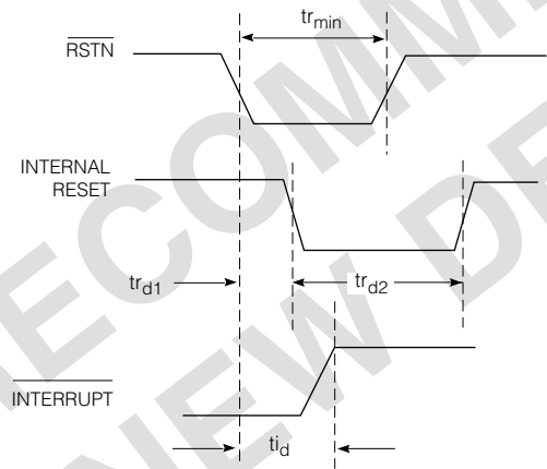
Fig. 2b Reset and Interrupt Timing
