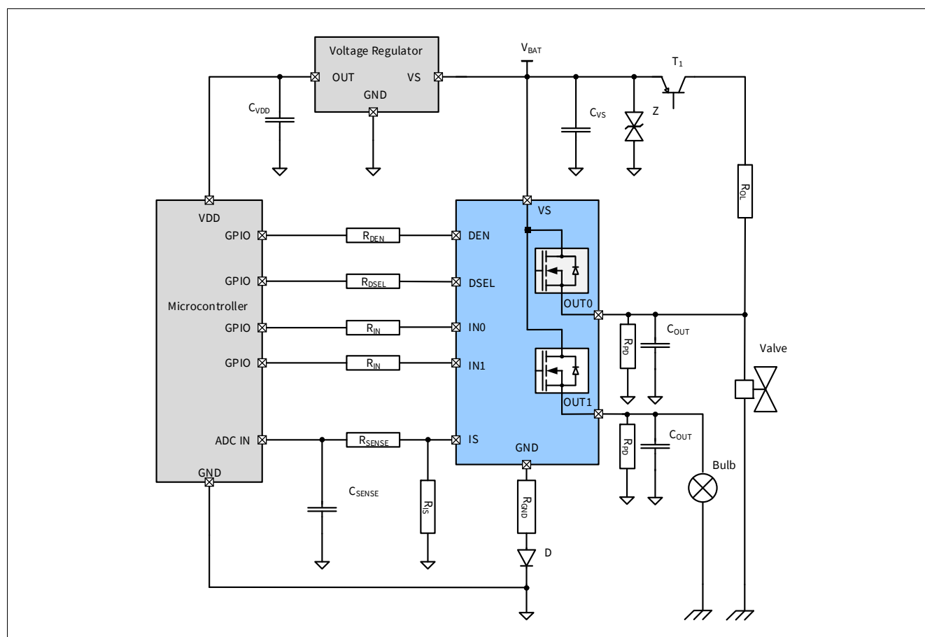
Application Diagram with BTT6030-2ERA
