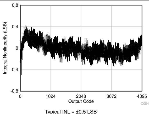
Figure 7-6. Typical INL
