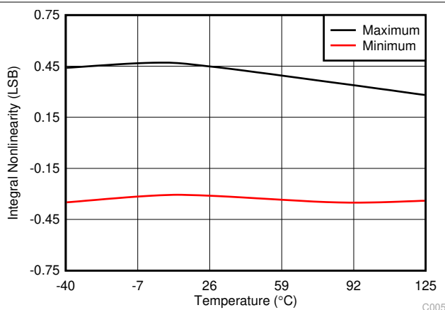
Figure 7-6. Typical INL
