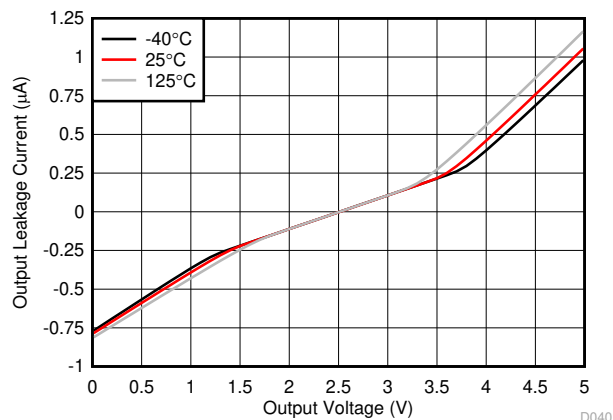
Figure 6-31. Output Leakage vs. Output Voltage (A1, A2, and A3 Devices)
