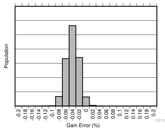
Figure 6-5. Gain Error Production Distribution A1 devices
