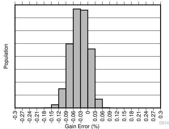
Figure 6-6. Gain Error Production Distribution A2, A3, and A4 devices
