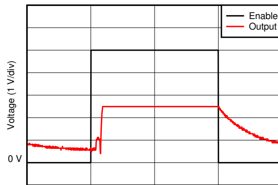
Figure 6-26. Start-Up Response
