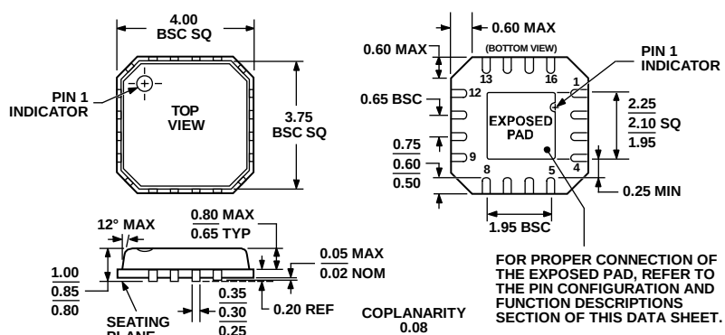
Figure 45.16-Lead Lead Frame Chip Scale Package [LFCSP_VQ] 4 mm × 4 mm Body, Very Thin Quad (CP-16-4)
