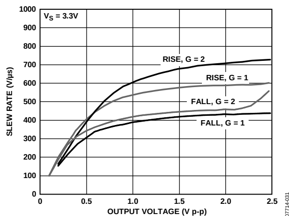
Figure 31. Slew Rate vs. Output Voltage, V_S = 3.3\text{ V}
