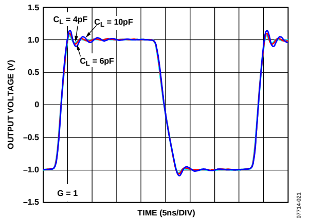
Figure 21. Large Signal Transient Response vs. Capacitive Load
