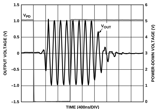
Figure 32. Enable/Power-Down Time
