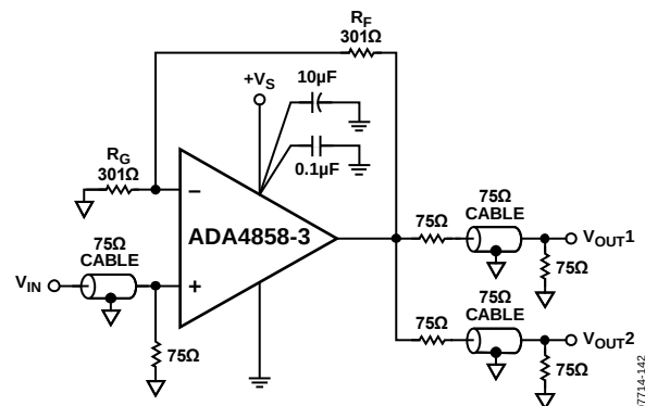
Figure 41. Video Driver Schematic for Two Video Loads
