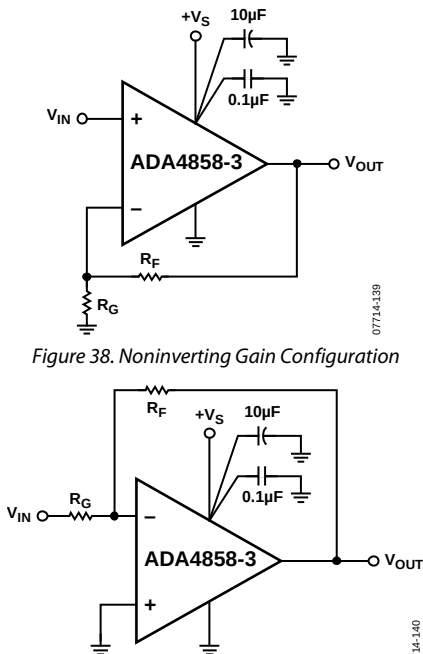
Figure 39. Inverting Gain Configuration
