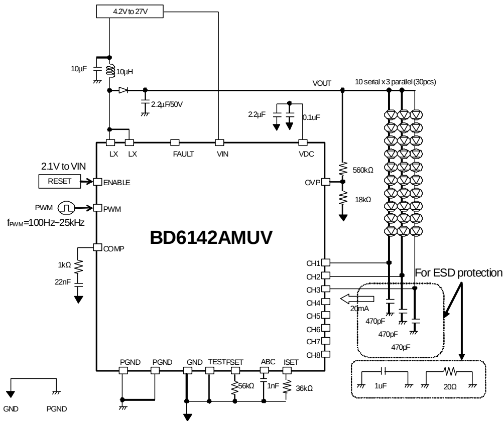
Figure 40. Application example of 10inch panel
