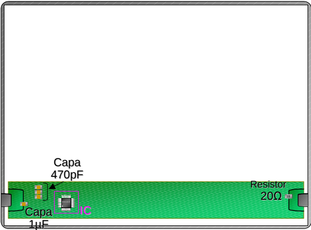
Figure 41. Layout example for ESD protection
