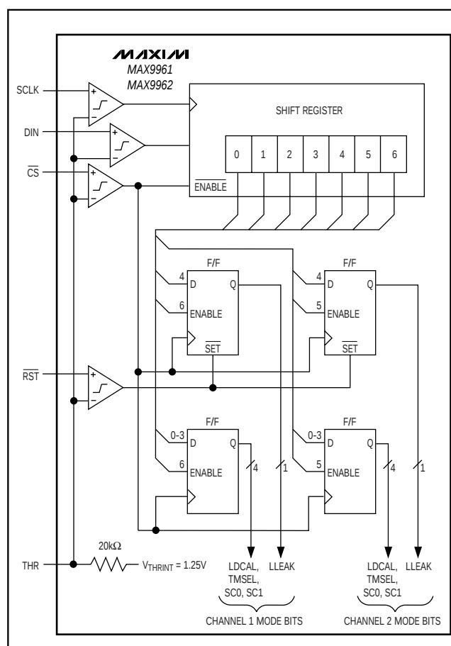
Figure 5. Serial Interface
