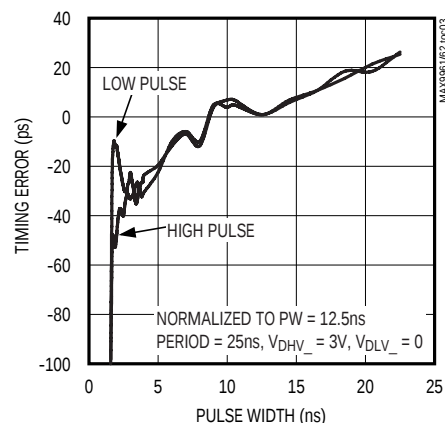
DRIVER TRAILING-EDGE TIMING ERROR vs. PULSE WIDTH
