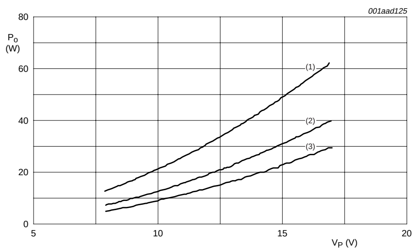
V_P = 14.4 V; R_L = 4 \Omega . (1) P_{o(max)} . (2) THD = 10 %. (3) THD = 0.5 %. Fig 21. Output power as a function of supply voltage
