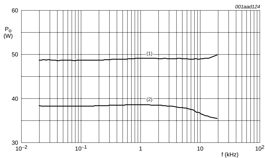
V_P = 14.4 V; R_L = 2 \Omega . (1) THD = 10 %. (2) THD = 0.5 %. Fig 20. Output power as a function of frequency
