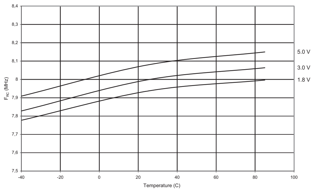
Figure 21-163. Calibrated 8 MHz RC Oscillator Frequency vs. Temperature
