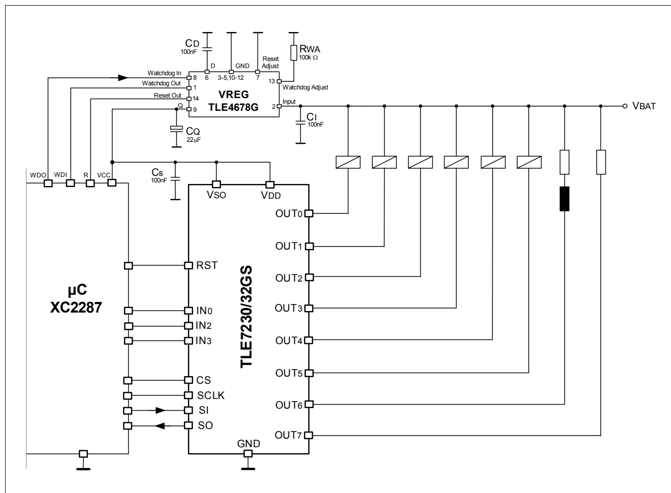
Figure 16 Application Circuit
