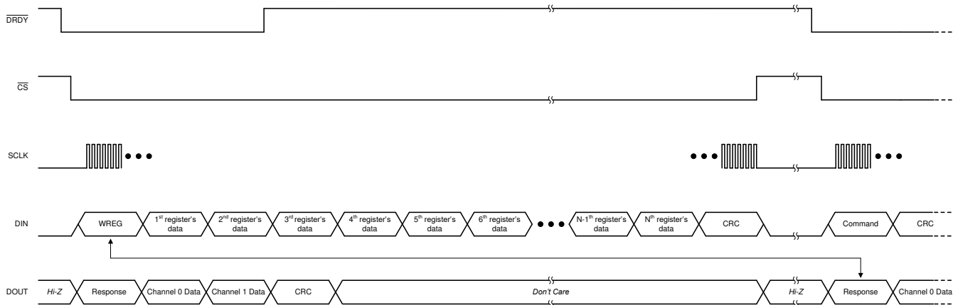
Figure 8-23. Writing Registers
