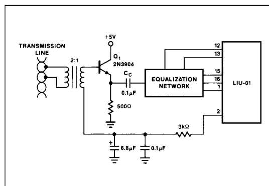
FIGURE 18: Emitter-follower Q_1 acts as buffer between the equalization network and the transmission line while operating from only a +5V supply.
