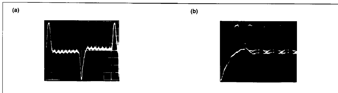
FIGURE 16: The LIU-01's preamplifier output, pin #1, should produce half-sinusoidal pulses of recovered data signal when properly equalized for the transmission line. The circuit of Figure 13 has excellent response as shown here receiving at 6000 ft. a 1-of-9 pattern, a, and a QRSS pattern, b.
