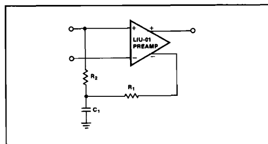
FIGURE 3: Preamp self-biasing for use with AC coupled, balanced bipolar signals.
